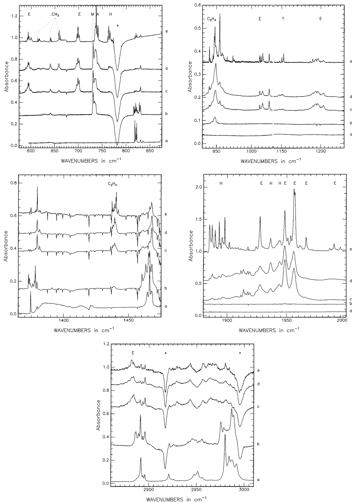
Figure 4. (a) \text{C}_2\text{H}_6/\text{Ar} 1/1000 deposited at 25 K, spectrum at 12 K, 0.8 mmol. (b)–(e) Dimethylmercury/Ar (1/2500) sample deposited at 12 K, spectra at 12 K, 8 mmol. Difference spectra (the reference spectrum is dimethylmercury before irradiation shown by *). Symbols: H for \text{HgH}_2 , E for \text{C}_2\text{H}_5\text{HgH} , A for acetylene, M for \text{CH}_3\cdots\text{Hg} . (b) After irradiation, 18 000 pulses, with a 2 mJ ArF laser (193 nm). (c) Sample (b) irradiated further with a KrF laser (750 pulses, 6 mJ). (d) Sample (c) irradiated with 3000 more KrF pulses. (e) Sample (d) after 15 min annealing at 34 K.
