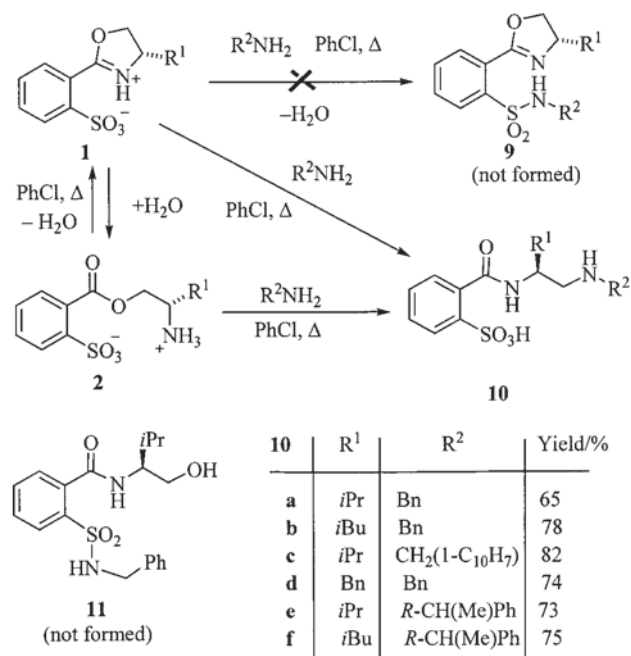
Scheme 4. Attempted preparation of sulfonamides via 1 or 2 .
