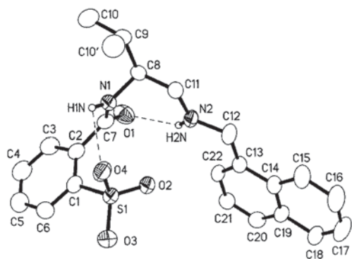
Figure 5. Molecular structure of 10c showing intramolecular hydrogen bonding. Selected H-bond lengths (Å) and angles ( ^{\circ} ): N(1)–H(1)N \cdots O(4), H(1)N \cdots O(4) 2.45, N(1) \cdots O(4) 2.965(4), N(2)–H(2)N \cdots O(1), H(2)N \cdots O1 2.34, N(2) \cdots O(1) 3.077(4), N(1)–H(1)N \cdots O(4) 118, N(2)–H(2)N \cdots O(1) 141.
