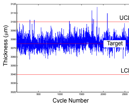
Fig. 9. Unloading thickness performance of the ADAC tuned controller
