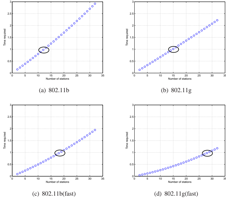
Figure 8 Time used on the medium: actual time (second) needed for total game traffic transmission in one second versus the number of players for different 802.11 networks. A circle is drawn in each sub-figure to highlight the limit at 1
