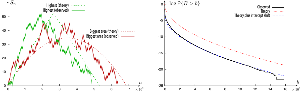
Figure 3: Bernoulli \{-1, +1\} increments with P(X_1 = -1) = 0.6 , P(X_1 = +1) = 0.4 . Simulated results from ten billion paths. (Left panel) Four paths displayed. Simulated path with largest swept area 15,825 and, conditioned on that area, most likely path to give rise to it predicted by Theorem 2, which is concave. For contrast, also shown is the simulated path that reaches the greatest height, 53, and, conditioned on that height, the most likely path to give rise to it as deduced from Theorem 1, which is piecewise linear. (Right panel) Logarithm of the empirical probability that area under busy period exceeds a given level compared with -K\sqrt{b} and, the linear shift -K\sqrt{b} + \kappa where \kappa is chosen to match the offset of the empirical observation
