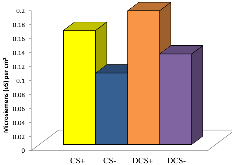
Figure 3.9. Mean increases in SCR (measured in \mu S microsiemens per cm^2 ) for learned threat and safety cues (CS+ & CS-) and also inferred threat and safety cues (DCS+ & DCS-) during Phase 2 (Probes) of Experiment 2.
