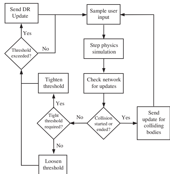
Figure 5: Flowchart of proposed authority scheme with adaptive threshold dead reckoning model.
