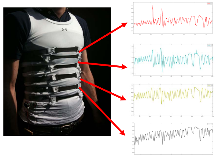
Figure 1. Respiratory shirt showing streams from several sensors.
