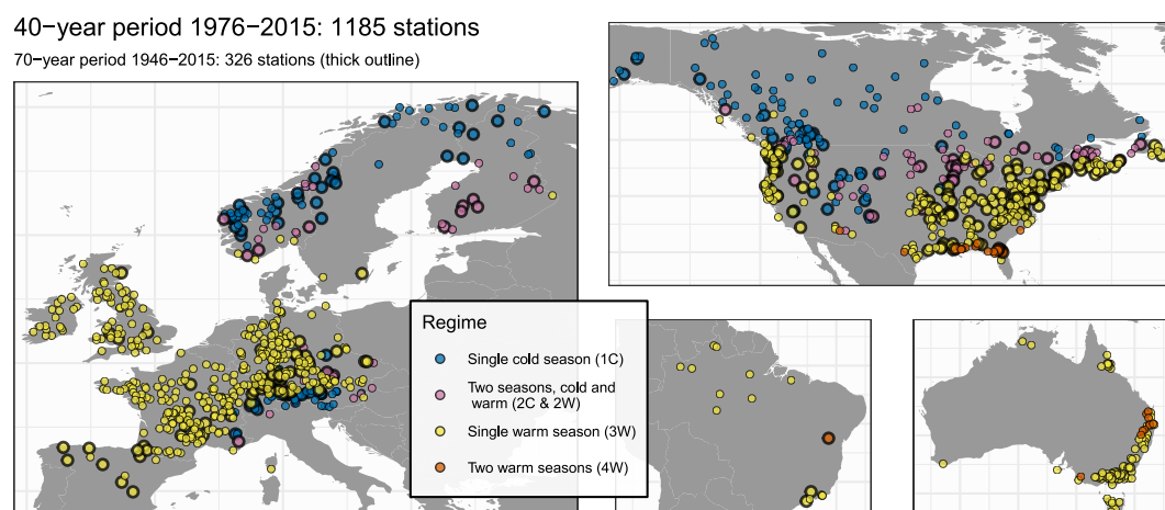
Figure 2. Distribution of the 40-year and 70-year study sites and their low-flow regime across four continents. The background grid has a spacing of 5^\circ latitude and longitude. Thin outlines on the symbols indicate sites with record from 1976 to 2015 while thick outlines indicate ones with record from 1946 to 2015.
