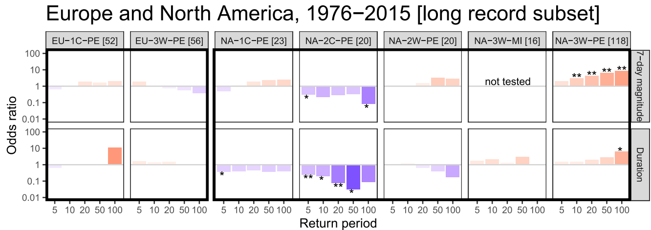
Figure 13. Trends from 1976 to 2015 in the group occurrence rate of extreme low streamflows (grouped by low-flow regime, streamflow permanence, and continent), using a subset of stations with records from 1946 to 2015. Red bars with two asterisks indicate significant ( p < 0.05 ) group increases while blue indicates decreases. Trend magnitude is expressed with the odds ratio. Continents: EU, Europe; NA, North America. See Figure 6 caption for additional explanation.
