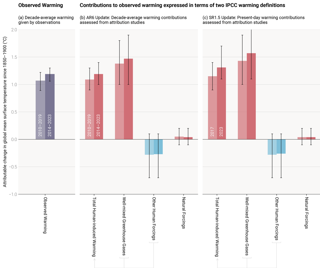
Figure 7. Updated assessed contributions to observed warming relative to 1850–1900; see AR6 WGI SPM.2. Results for all time periods in this figure are calculated using updated datasets and methods. To show how these updates have affected the previous assessments, the 2010–2019 decade-average assessed results repeat the AR6 2010–2019 assessment, and the 2017 single-year assessed results repeat the SR1.5 2017 assessment. The 2014–2023 decade-average and 2023 single-year results are this year’s updated assessments for AR6 and SR1.5, respectively. For each double bar, the lighter and darker shading refers to the earlier and later period, respectively. Panel (a) shows updated observed global warming from Sect. 6, expressed as total global mean surface temperature (GMST), due to both anthropogenic and natural influences. Whiskers give the very likely range. Panels (b) and (c) show updated assessed contributions to warming, expressed as global mean surface temperature (GMST), from natural forcings and total human-induced forcings, which in turn consist of contributions from well-mixed greenhouse gases and other human forcings. Whiskers give the likely range.
