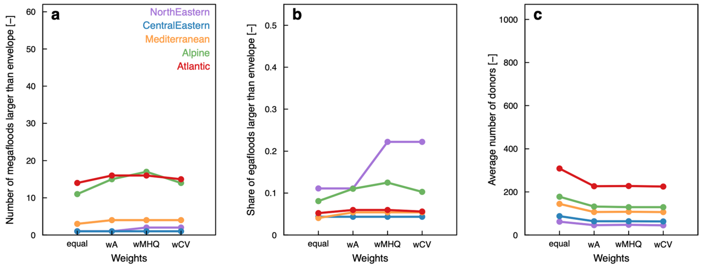
Extended Data Fig. 6 | Sensitivity of results to the weights used for estimating distance D. (a) Number and (b) fraction of megaflods larger than envelope for four weight combinations: equal weights ('equal', \alpha = \beta = \gamma = 1 ), double weight for Area ('wA', \alpha = 2 ), double weight for mean annual flood ('wMHQ', \beta = 2 ), double weight for CV ('wCV', \gamma = 2 ). (c) Average number of donor catchments for the four weight combinations. Colours indicate the five alternative regions of Extended Data Fig. 4a.
