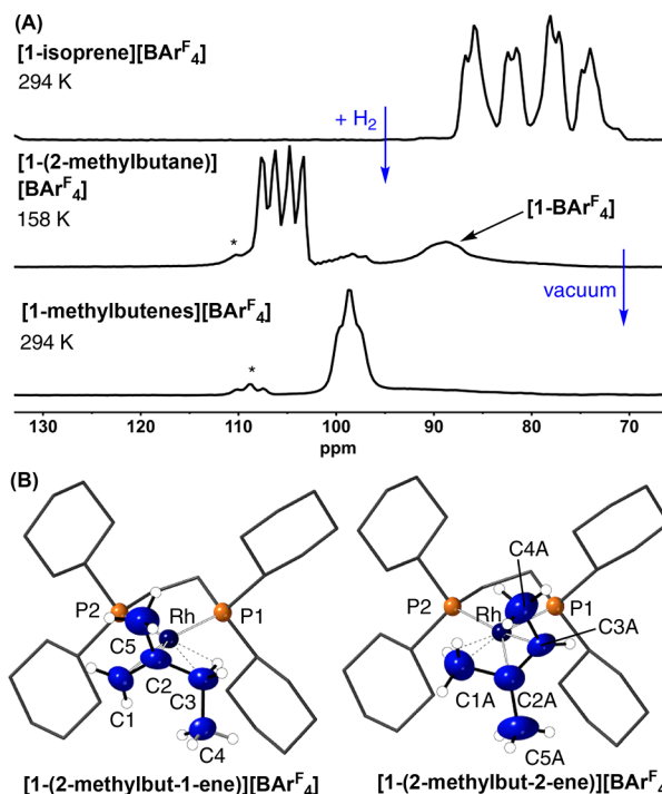
Figure 5. (A) 31 P{ 1 H} SSNMR spectra of the sequential SC–SC transformation of [1-isoprene][BARF 4 ] to [1-(2-methylbutane)][BARF 4 ] and [1-(2-methylbut-1-ene)][BARF 4 ]/[1-(2-methylbut-2-ene)][BARF 4 ]. Asterisks indicate an unidentified product. (B) Solid-state molecular structures of the dehydrogenation products. Both 50:50 disordered components are shown, with 30% displacement ellipsoids. Selected bond distances (Å) and angle (deg) for [1-(2-methylbut-1-ene)][BARF 4 ]: Rh–C1, 2.23(2); Rh–C2, 2.12(2); Rh–C3, 2.36(2); C1–C2, 1.39(3); C2–C5, 1.53(3); C2–C3, 1.52(3); ∑ angles around C2, 359.9. Selected bond distances (Å) and angle (deg) for [1-(2-methylbut-2-ene)][BARF 4 ]: Rh–C2A, 2.11(2); Rh–C3A, 2.3(2); Rh–C1A, 2.41(3); C1A–C2A, 1.54(3); C2A–C5A, 1.55(4); C2A–C3A, 1.37(3); ∑ angles around C2A, 359.9°.
