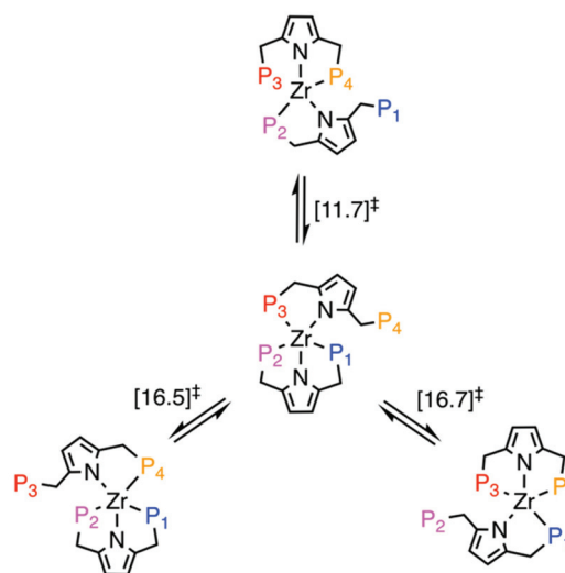
Fig. 5 Summary of ligand exchange pathways for [ \text{PNP}^{\text{Me}}\text{H} ] _{2}\text{ZrCl}_{2} . Free Energies (BP86/def2-TZVP corrected for toluene solvent) of the rate-determining step in each pathway are given in \text{kcal mol}^{-1} .
