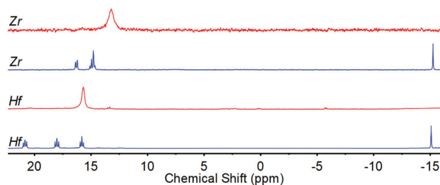
Fig. 4 The variable temperature ^{31}\text{P}\{^1\text{H}\} NMR of [ \text{PNP}^{\text{Ph}}\text{H} ] _{2}\text{MCl}_{2} (M = Zr, Hf) in d_8 -toluene. Red spectrum is measured at 298 K, blue spectrum is measured at 203 K. For spectra at 10 K increments see ESI.†
