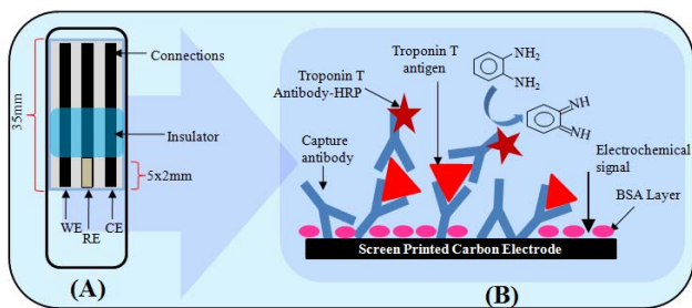
Fig. 1. (A) Screen printed carbon working electrode (WE) Ag/AgCl reference (RE) and carbon counter electrode (CE). (B) Working principle of the electrochemical immunosensor.
