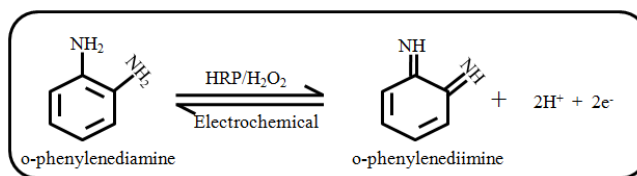
Scheme 2. Oxidation of o-phenylenediamine to o-phenylenediimine by HRP enzyme (forward reaction) and electrochemical reduction of o-phenylenediimine at the immunoelectrode surface by CV (backward reaction).
