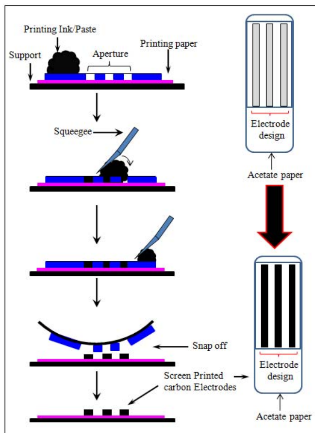
Scheme 1. Schematic showing the stages involved in the electrode printing process.
