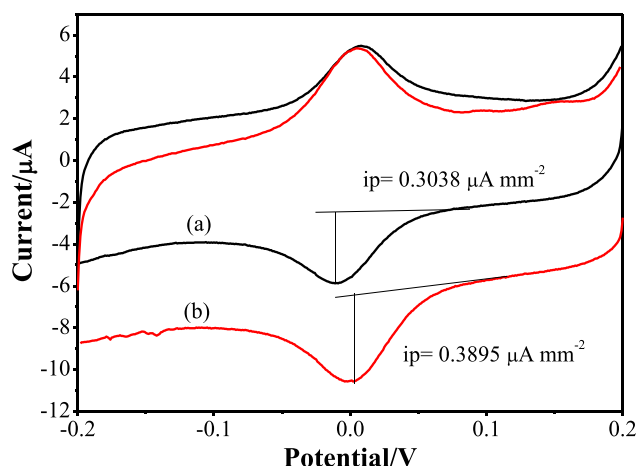
Fig 5. Cyclic voltammogram of modified SPE in 1 mM o-phenylenediamine /H 2 O 2 in phosphate buffer pH 6 vs. Ag/AgCl reference electrode at 100 mVs -1 , (a) SPE/Ab/BSA/Ab-HRP, and (b) SPE/Ab/BSA/cTnT (1000 ng ml -1 )/Ab-HRP.
