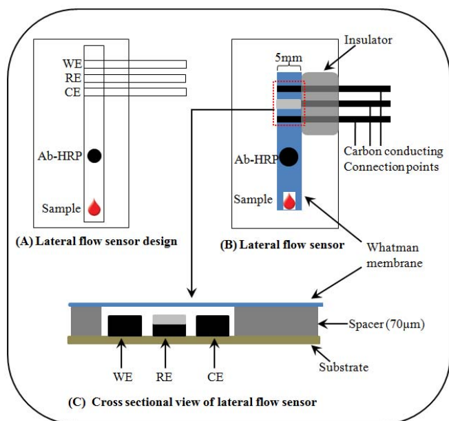
Fig. 2. Lateral flow immunosensor fabricated using screen printed carbon electrodes.
