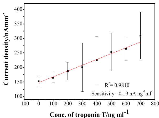
Fig 8. Calibration curve for Troponin T using the electrochemical lateral flow immunosensor, over a concentration range of 100-700 ng ml -1 (n=5 devices).
