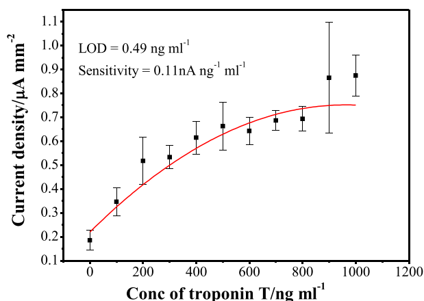
Fig 6. Calibration plots shows current density vs. concentration of troponin T detected at the SPE surface (n=5). Limit of detection = 0.49 ng ml -1 .
