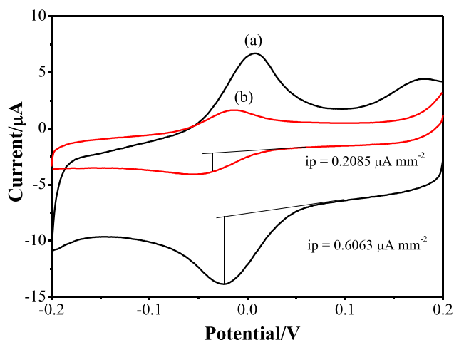
Fig. 4. Cyclic voltammogram of in-house screen printed carbon electrode (a) SPE/HRP-Ab, (b) SPE/BSA/HRP-Ab in 1 mM o-phenylenediamine/H 2 O 2 in phosphate buffer, pH 6 at 100 mV s -1 vs. Ag/AgCl reference electrode.
