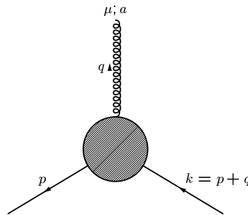
Figure 1: The quark–gluon vertex.
