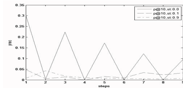
Fig. 2. Prec@10 for documents and images with CEDD facet
