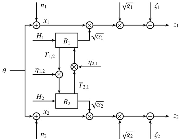
Fig. 1. System model for two sensors.
