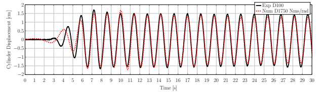
Figure 18: Numerical and experimental cylinder displacement for D_{num} = 1750\text{Nms/rad} and D_{exp} = 100
