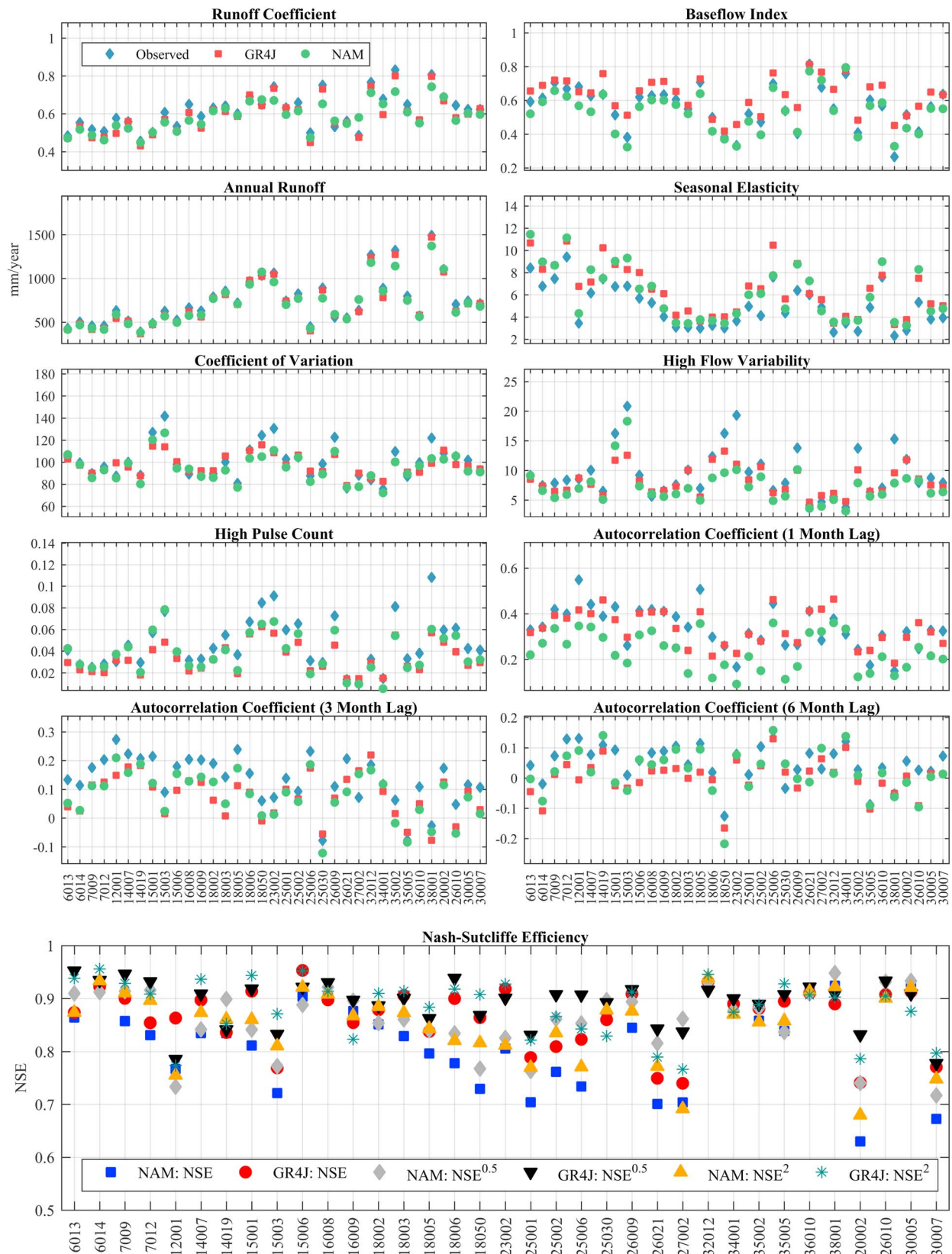
Figure 3. Observed and rainfall-runoff model (GR4J and NAM) simulated hydrological signatures estimated for each catchment using the period for which observed flow data are available. Also shown (lower panel) are the Nash Sutcliffe Efficiency (NSE) validation scores for each catchment and rainfall-runoff model.
