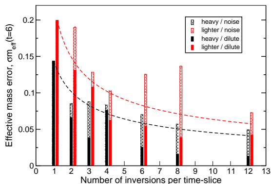
Figure 4. Equal cost test of the pion effective mass at timeslice 6.
